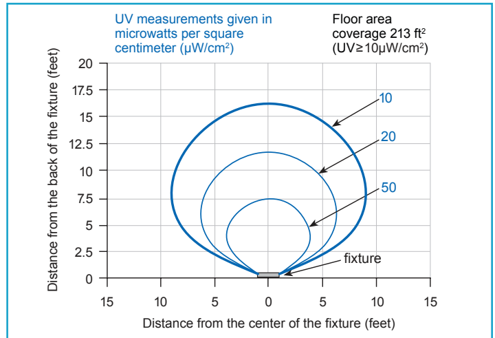
Coverage area of the Hygeaire® Model LIND24-EVO wall mounted fixture
