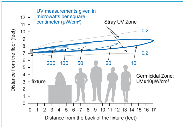
Distribution of UV rays from Hygeaire® Model LIND24-EVO wall mounted fixture
